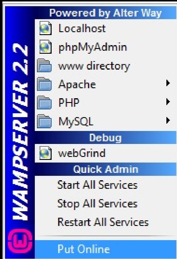
WAMP Server
